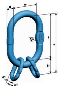
VMWP Oversize master link assembly
